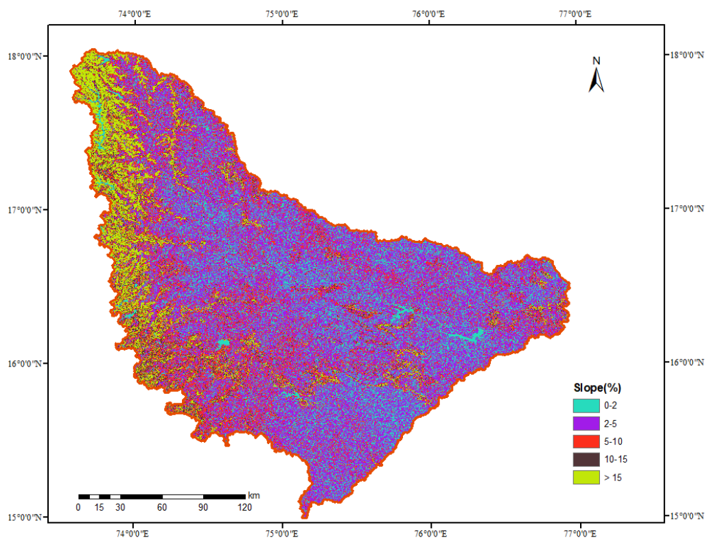
Fig. 5. Slope map of the study area
