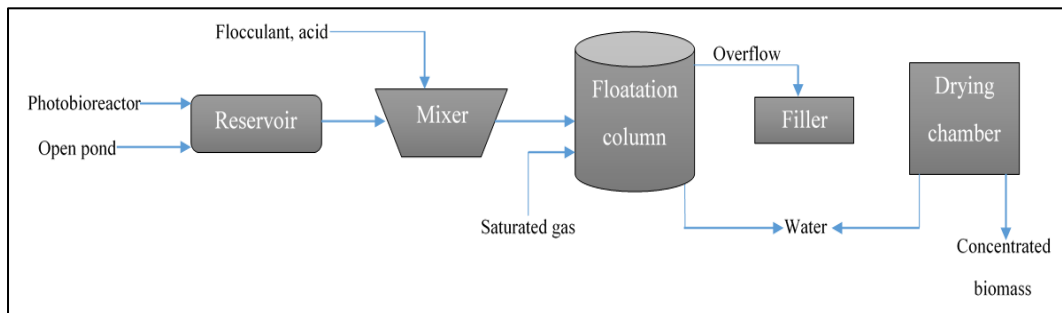
Fig. 4. The method and process of microalgae harvesting
