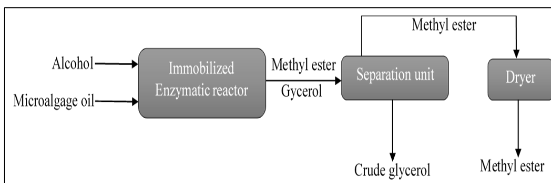
Fig. 5. A depiction of the immobilized transesterification process
