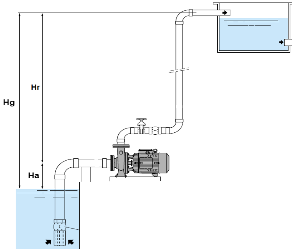
Fig. 3. Suction pump assembly
