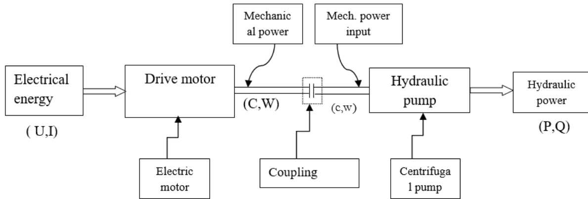
Fig. 7. Schematic diagram
