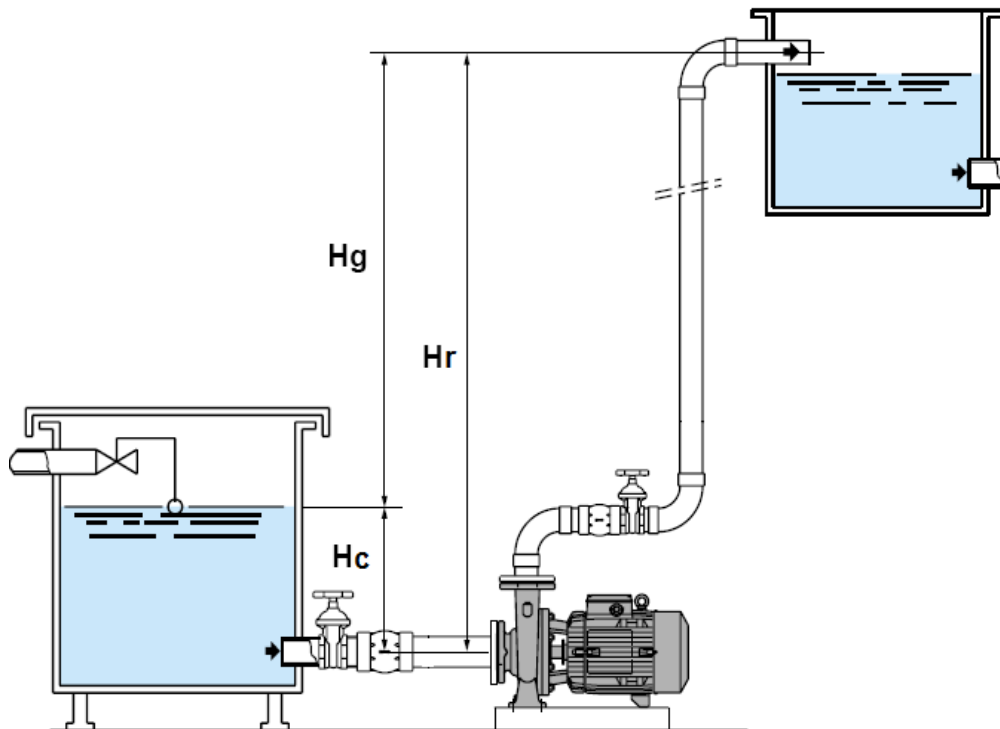
Fig. 2. Load pump assembly
