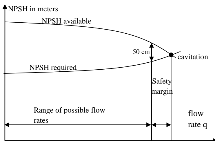
Fig. 4. Practical NPSH curves
