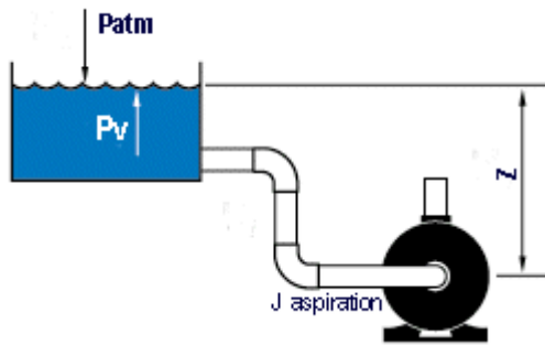
Fig. 5. Pump under load
