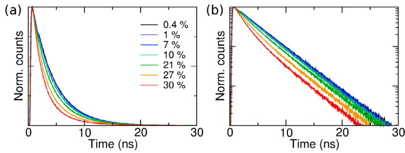
Figure 2. Photon pile-up of a fluorescein decay measured with a point detector; as the count rate increases, the initially monoexponential decay becomes shorter and non-exponential. The photon detection rate is indicated as % of the excitation repetition rate. (a) Linear scale, (b) semilogarithmic scale.
