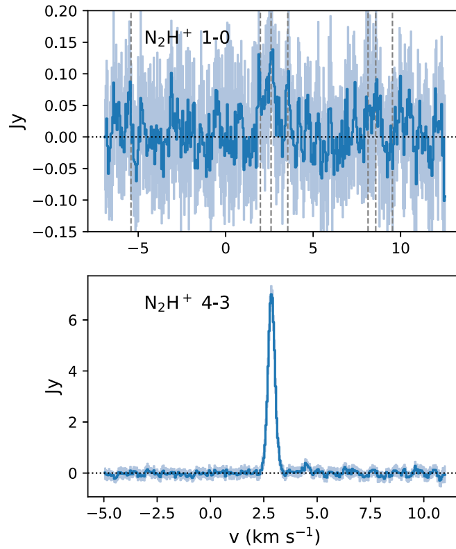
Figure 1. Spectra for the \text{N}_2\text{H}^+ J = 1-0 (top panel) and J = 4-3 (bottom panel) lines after deprojection, stacking, and averaging over a ring from 0''.8 to 2'' . Light shading indicates the 1\sigma uncertainty in each channel. Vertical dashed lines show the expected location of the 1-0 hyperfine lines.
