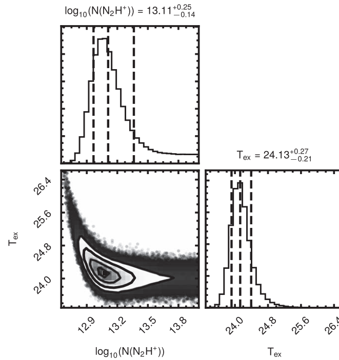
Figure 2. Posterior distributions from the rotation diagram analysis. Dashed lines indicate the 16th, 50th, and 84th percentiles.
