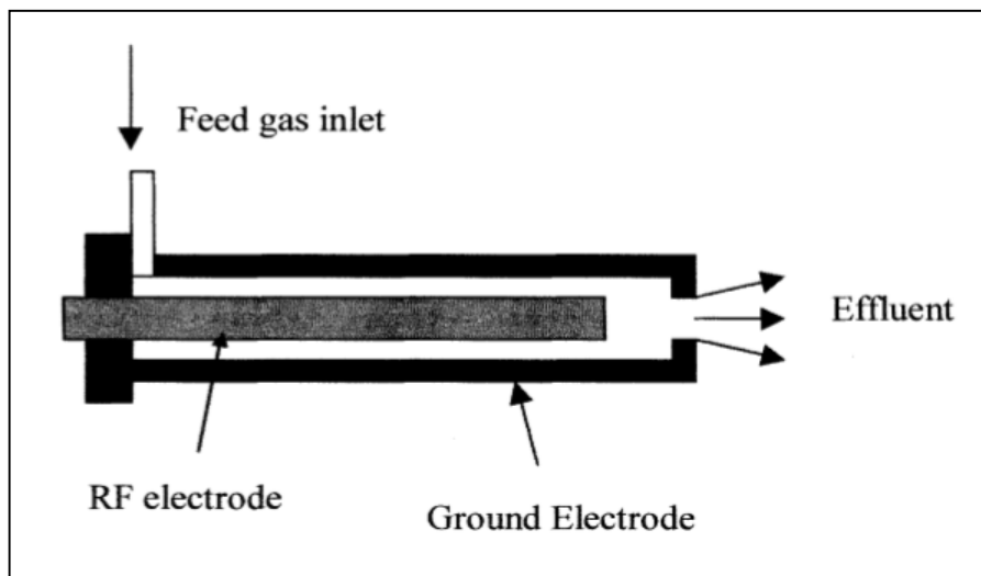
Fig. 3. Configuration of the atmospheric-pressure plasma jet (APPJ)
