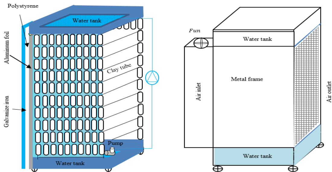
Fig. 1. Prototype of the terracotta tube evaporative cooler
