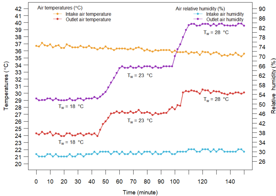
Fig. 7. Influence of water temperature on the outlet air temperature and humidity
