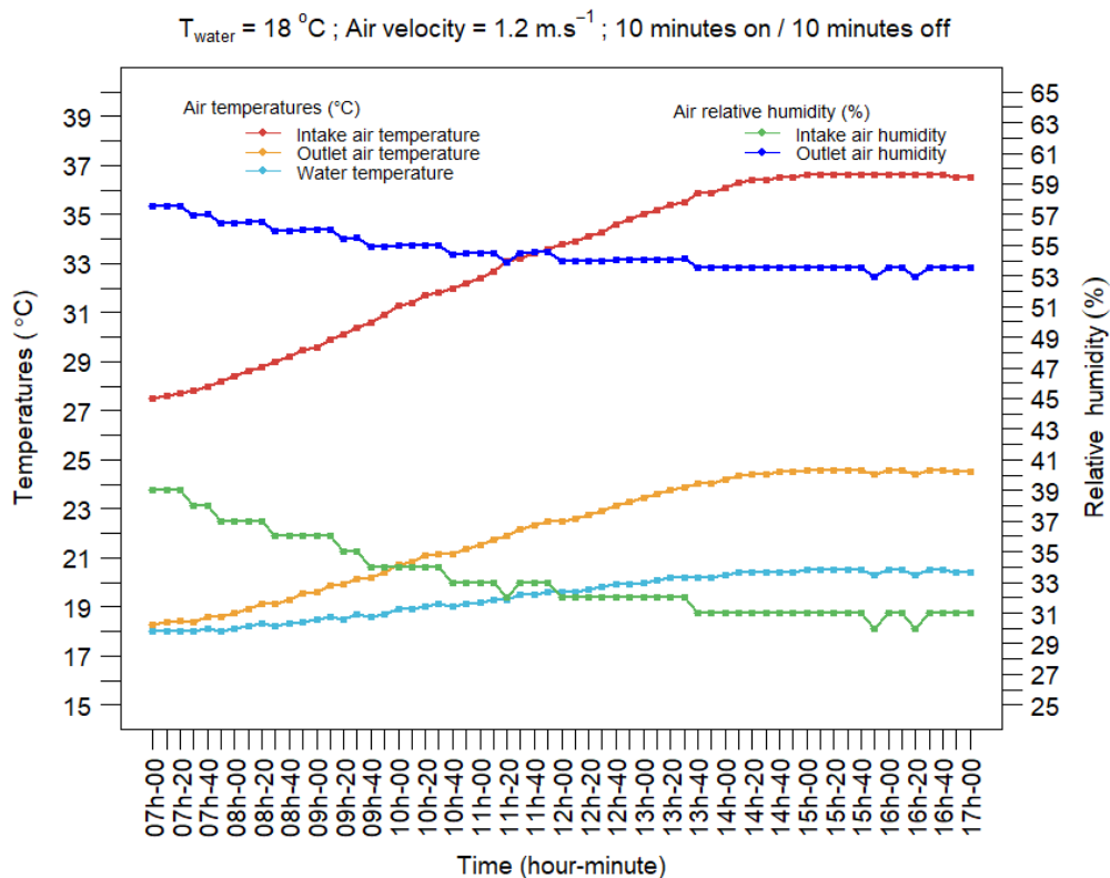
Fig. 8. The dynamic operating performance of the cooler
