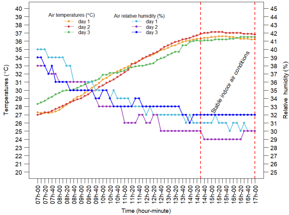
Fig. 5. Daily fluctuations of air temperature and humidity in the test room over three consecutive days
