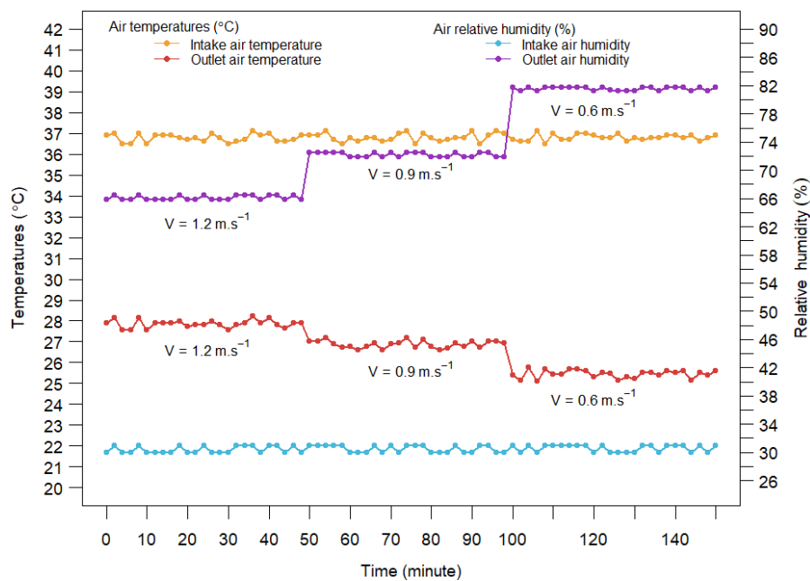
Fig. 6. Influence of intake air velocity on the outlet air temperature and humidity
