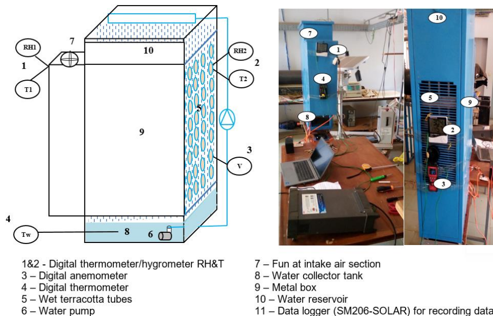
Fig. 4. Experimental setup
