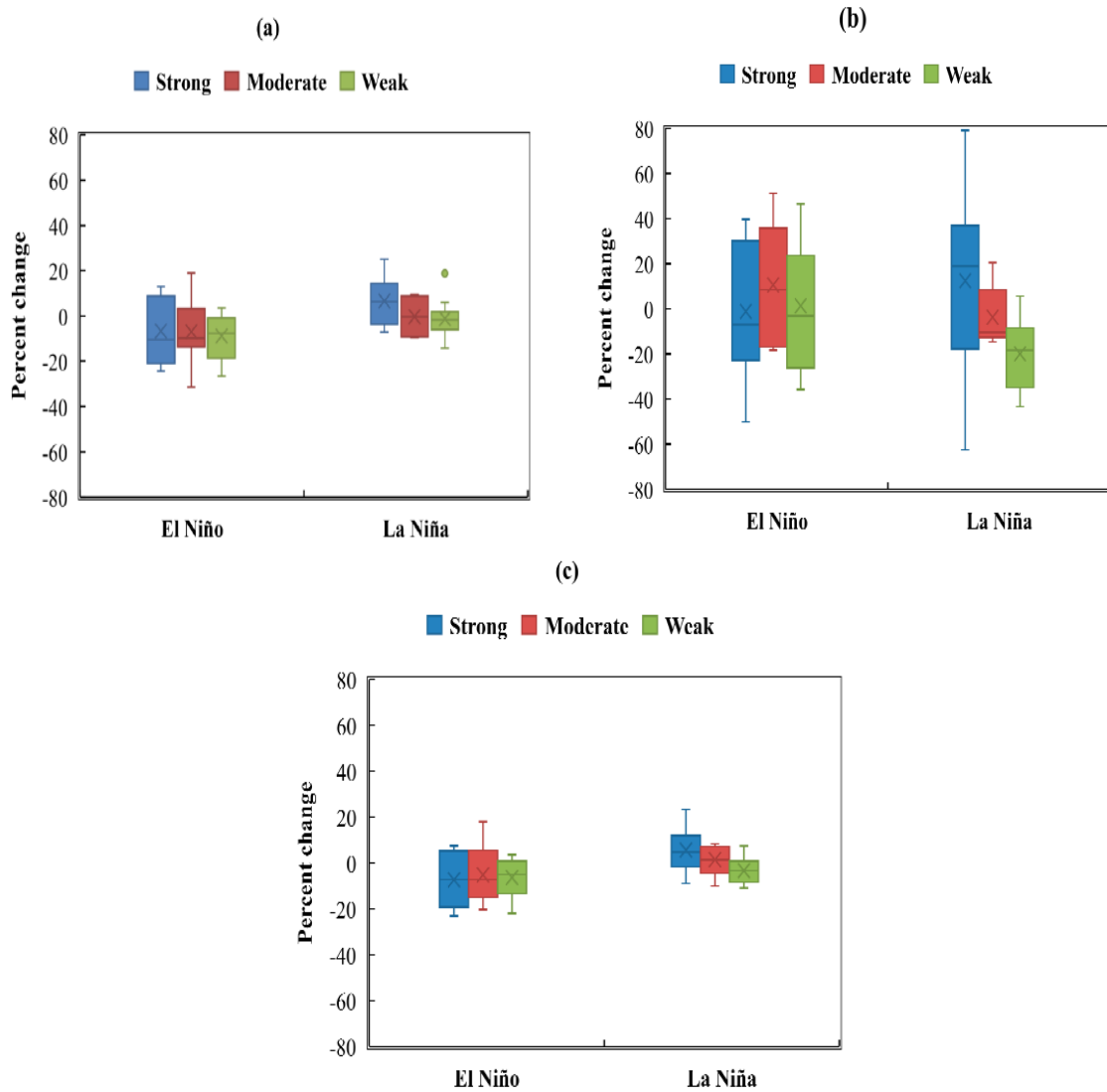
Fig. 3. Box plots depicting the percent change in (a) S-W monsoon, (b) N-E monsoon, and (c) annual rainfall during El Niño and La Niña years compared to normal years in Karnataka (1951–2014)
