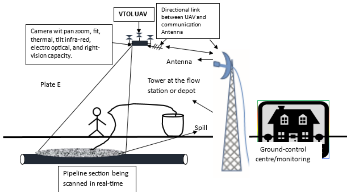
Fig. 1. Architectural diagram of Portable easily deployable VTOL
